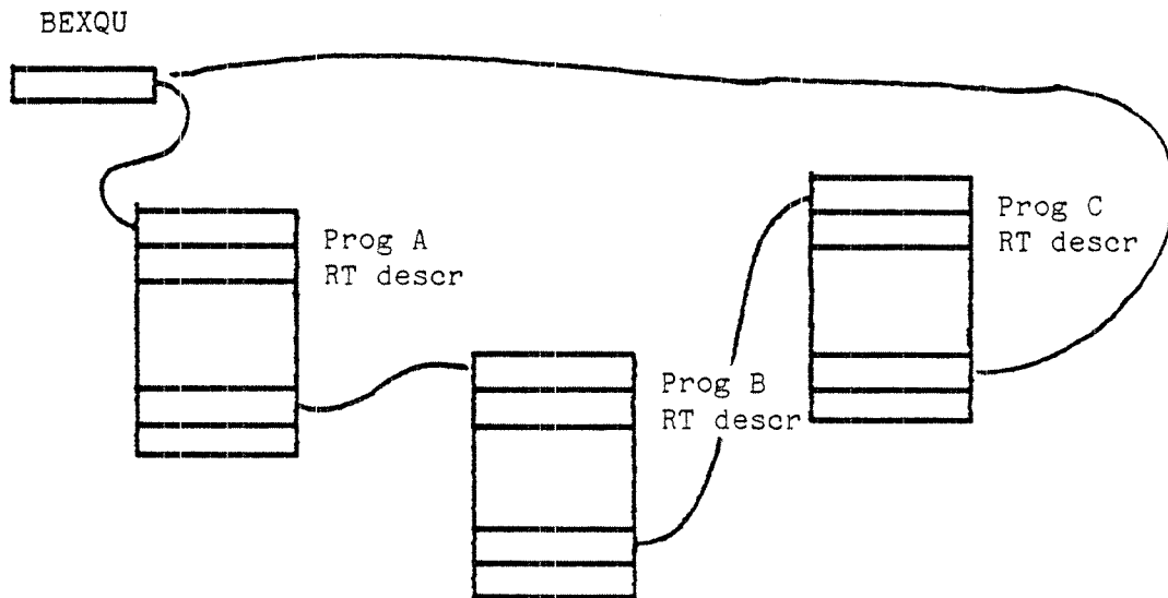
Fig. 10. Execution queue
