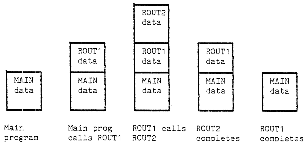
Fig. 33. Stack allocation
