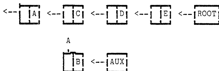
Fig. 21. B has been unlinked
