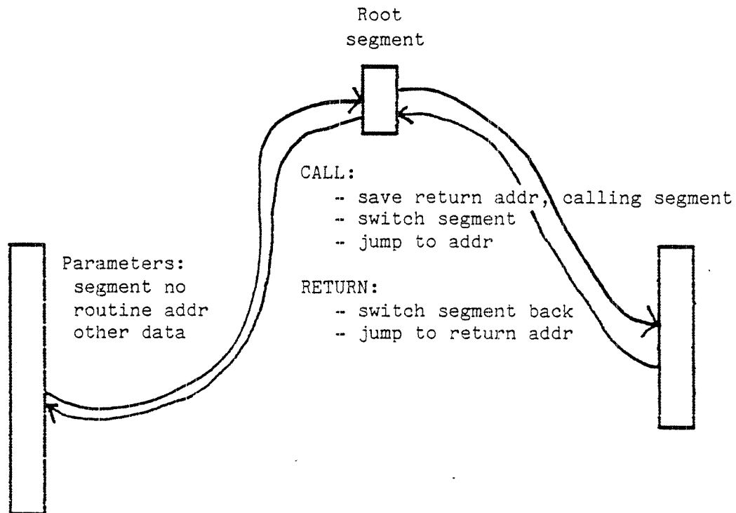
Fig. 32. Calling another segment via a root segment
