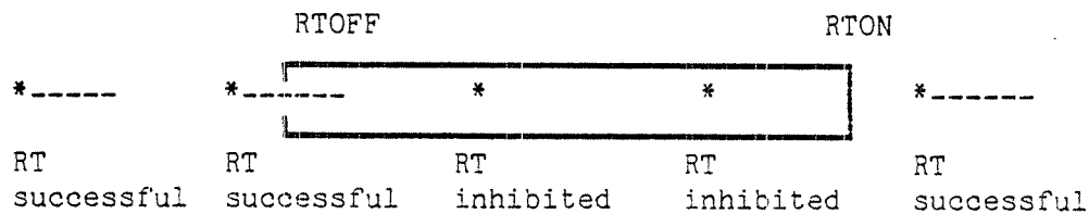
Fig. 17. MON RT inhibited in the RTOFF state
