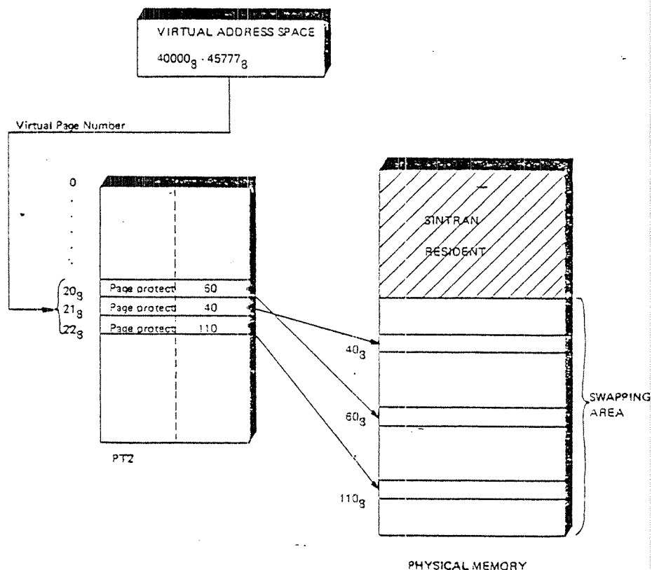
Fig. 1. Address translation
