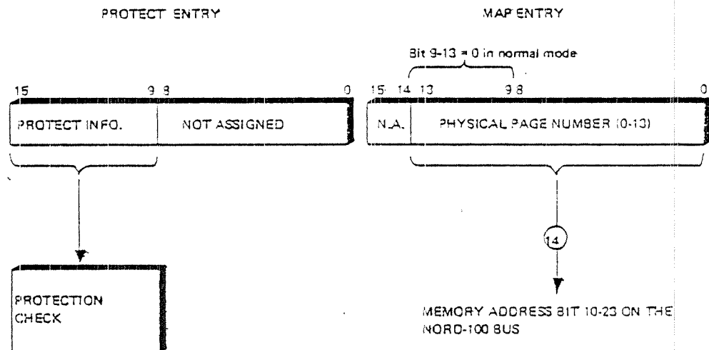
Fig. 3. ND-100 page table entry
