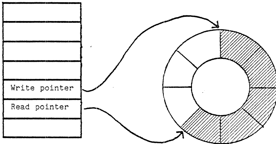
Fig. 24. Ring buffer and datafield
