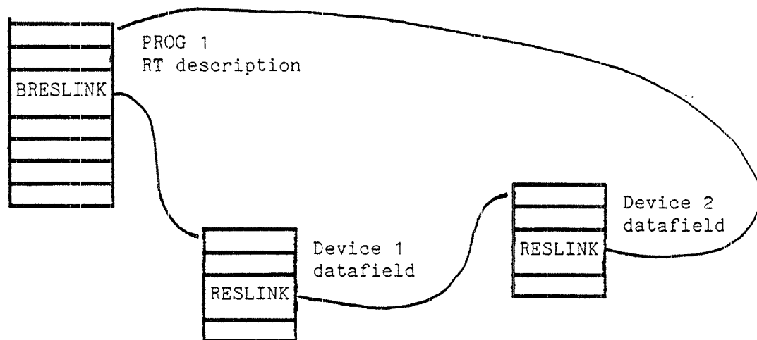
Fig. 12. Reservation queue
