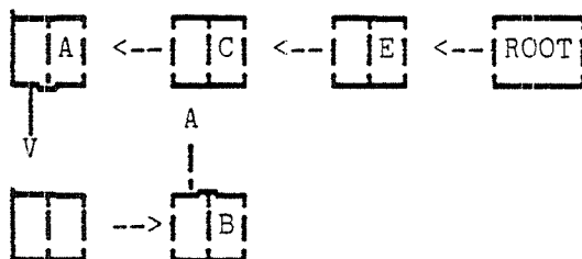
Fig. 23. An unintended loop
