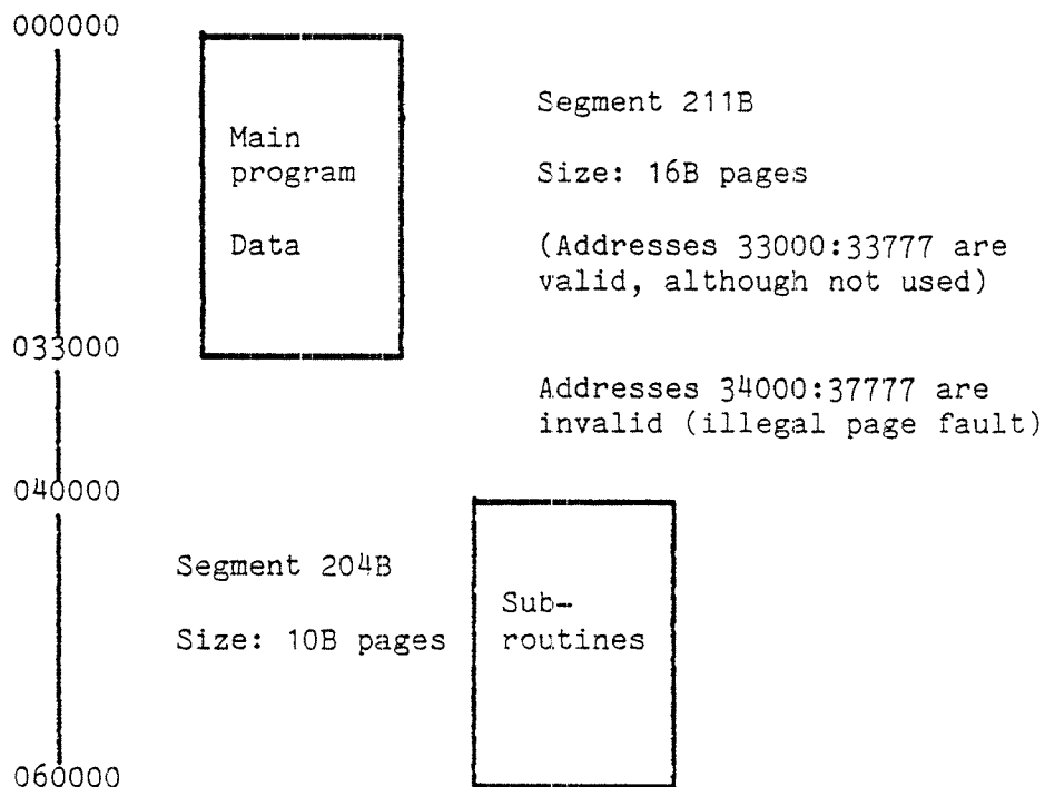
Fig. 14. Two segments used concurrently by a program
