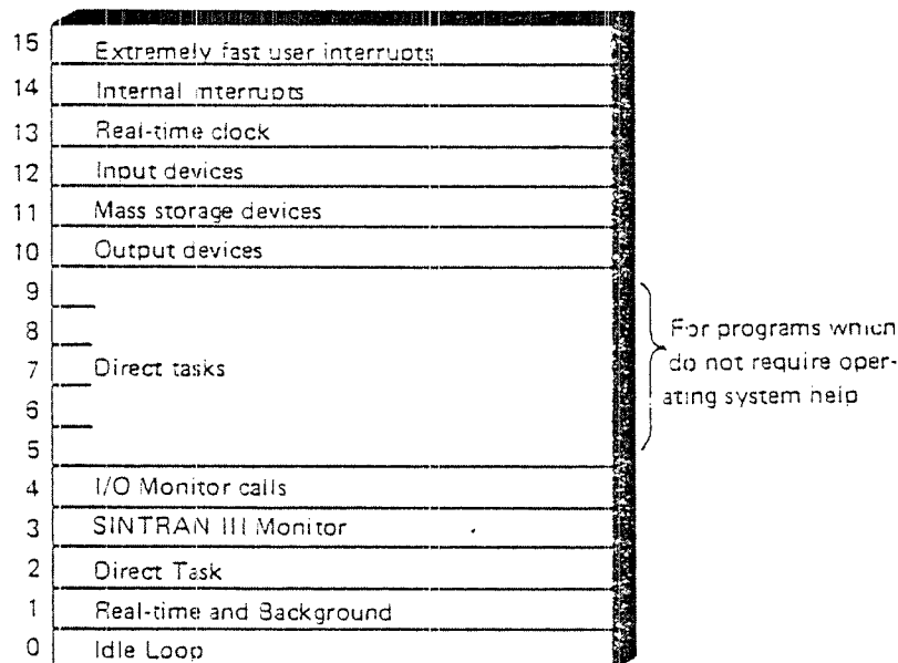
Fig. 8. Sintran interrupt level assignments
